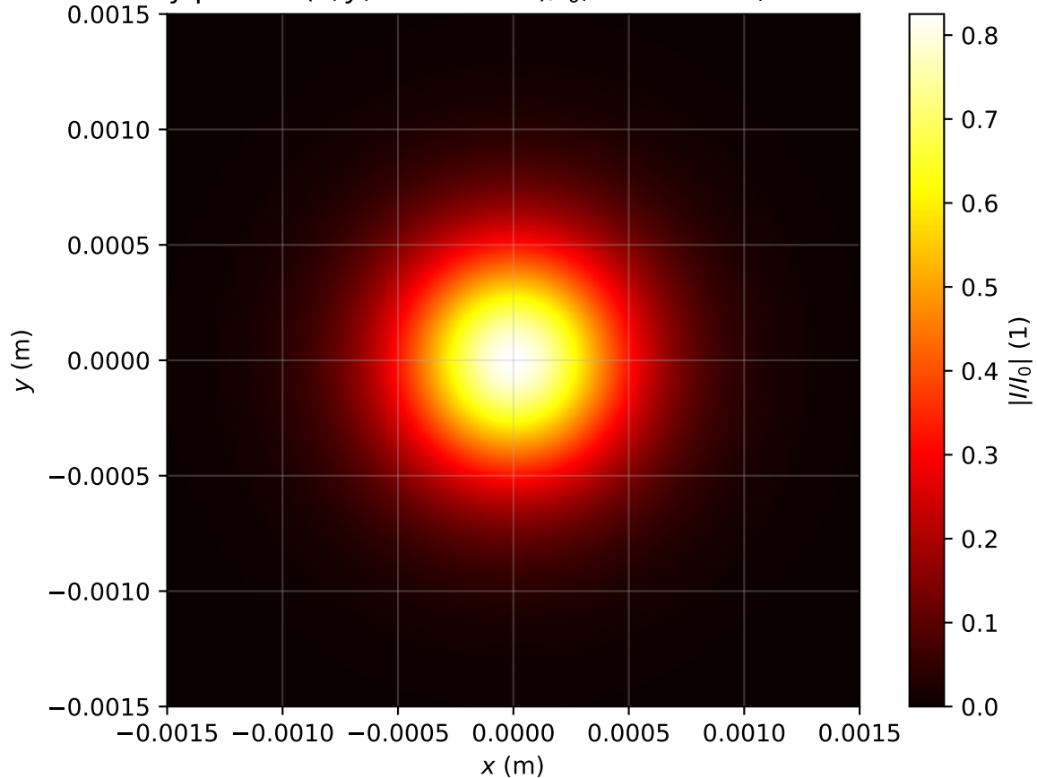
Intensity profile I(x, y, z = 1.990m)/I_0 , \text{Pin}=0.5\text{Pcr} , artificial time
